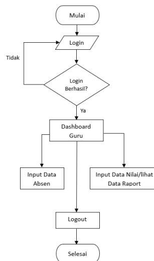
Gambar 6. Flowchart Guru
