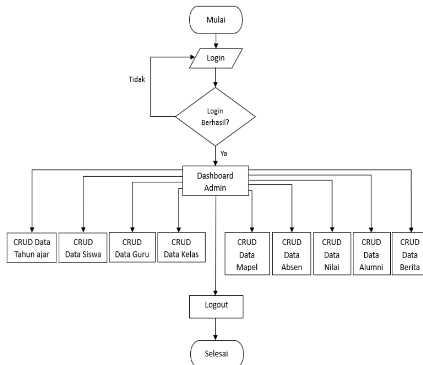
Gambar 5. Flowchart Admin
